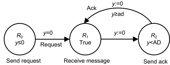
Fig. 3 An honest recipient model
