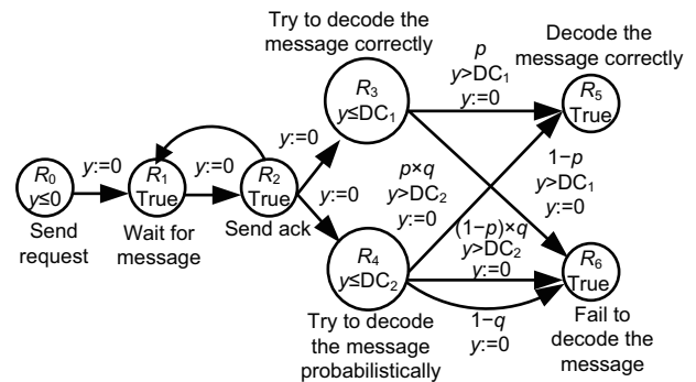
Fig. 5 A more powerful malicious recipient model
