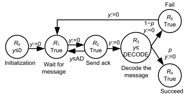
Fig. 4 A simple malicious recipient (SMR) model
