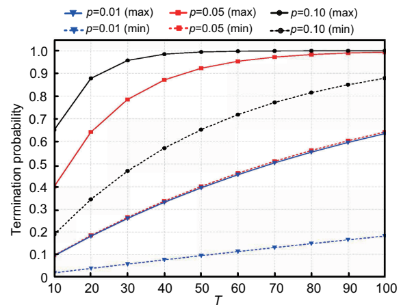
Fig. 7 Termination probability within T time units
