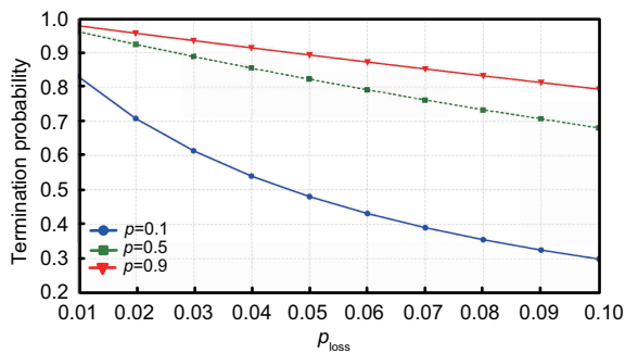
Fig. 6 Termination probability for a lossy channel
